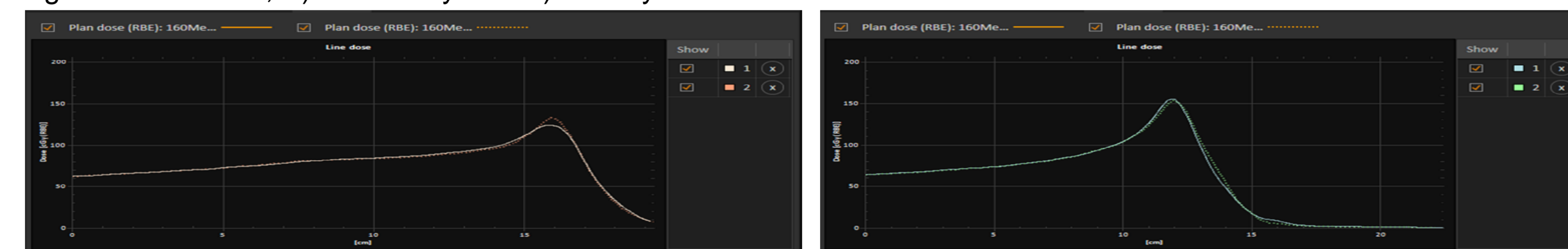
Figure 6. Dose profile perturbation at 160 MeV. A) current marker without (1) and with density override (2), B) RT-SPOT marker without (1) and with density override (2).
